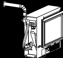
Up and back direct OR Up and back extended flueing
